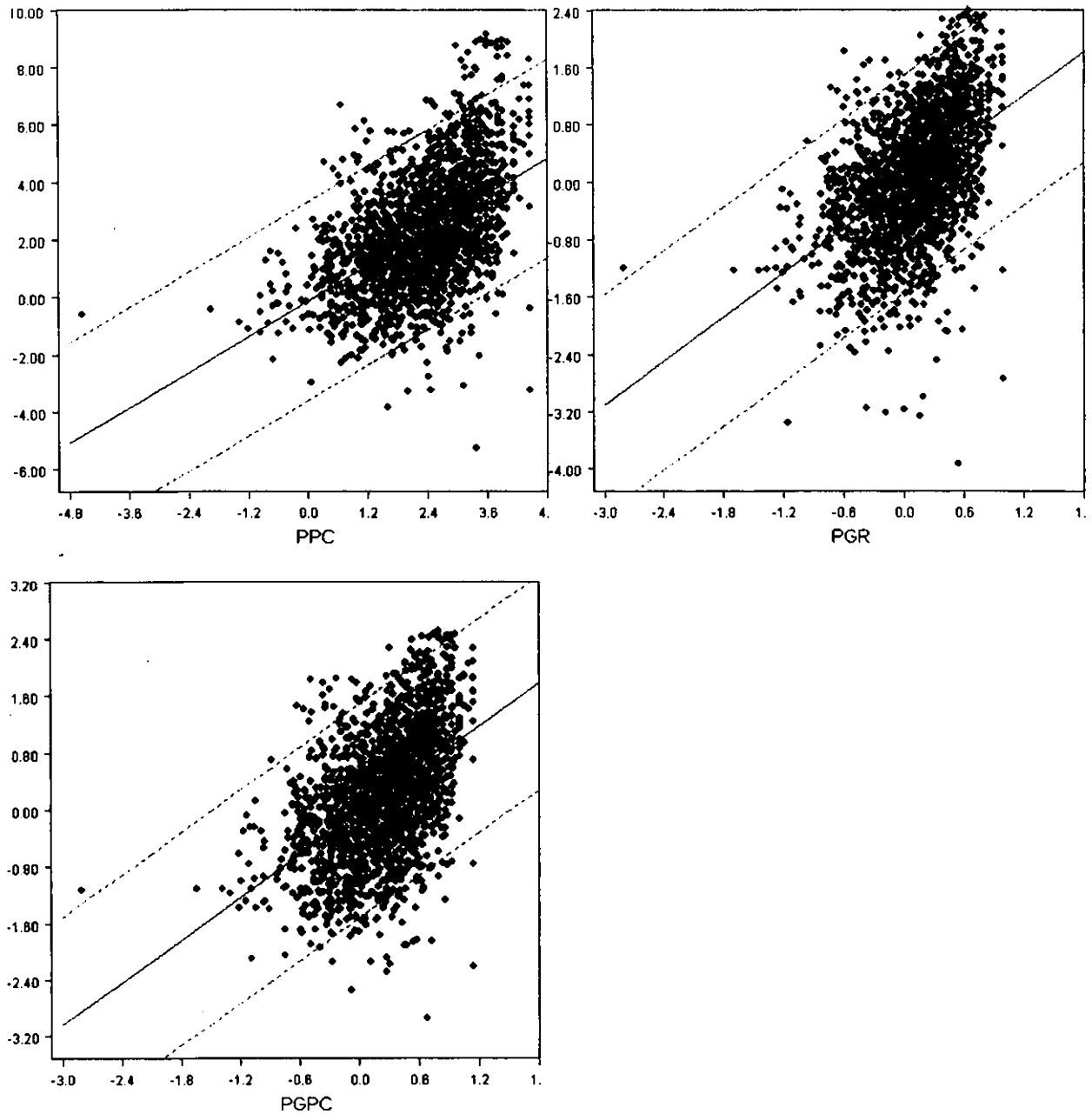
FIGURE 4. Scattered plot of cross-validated achievement measures on predicted achievement measures from preadmission variables for: upper left – Partial Credit adjusted GPA, upper right – Graded Response adjusted GPA, lower left – Generalized Partial Credit adjusted GPA.
